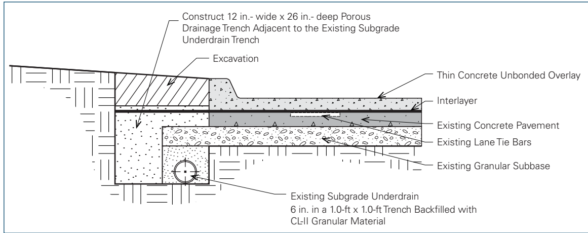
Figure 89. Drainage of separation layer (interlayer) into an existing underdrain system when existing curb is removed and replaced (source: Dan DeGraaf, Michigan Concrete Association)
