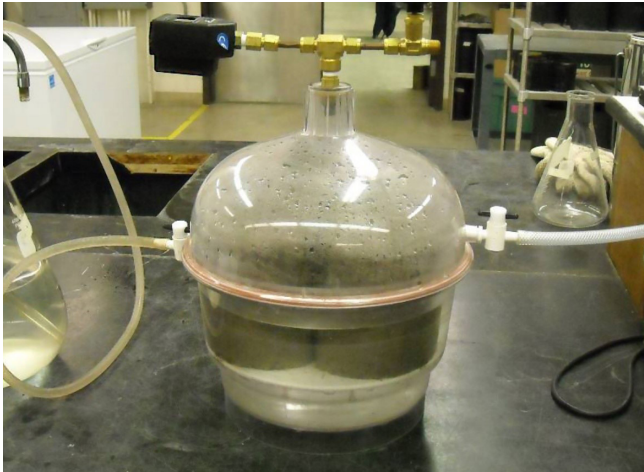
Figure 5.11. Vacuum saturation test
