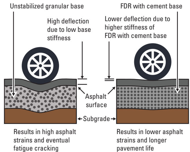
Figure 1.3. FDR with cement base reduces fatigue cracking compared to an unstabilized base
