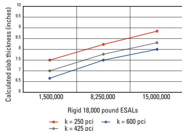
Figure 4.13. Calculated slab thickness for moderate volume roads, concrete flexural strength = 650 psi
