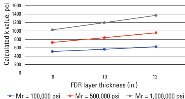
Figure 4.10. Composite k values, subgrade M_r = 7,000 psi
