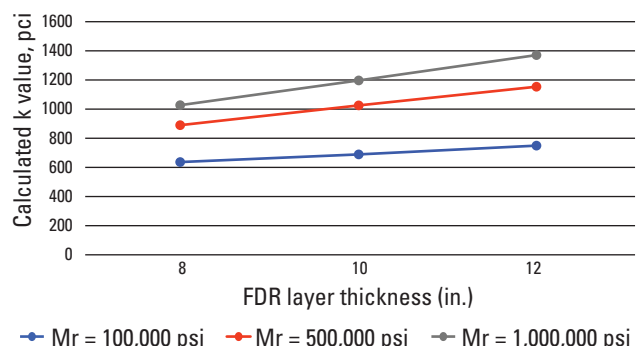
Figure 4.11. Composite k values, subgrade M_r = 9,000 psi
