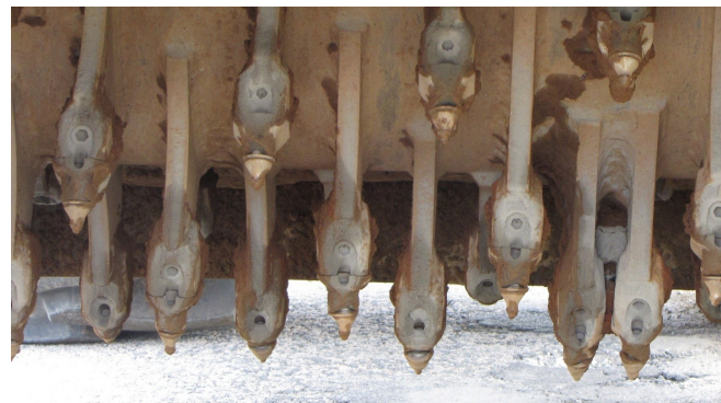
Figure 6.3. Roadway reclaimer cutting drum
